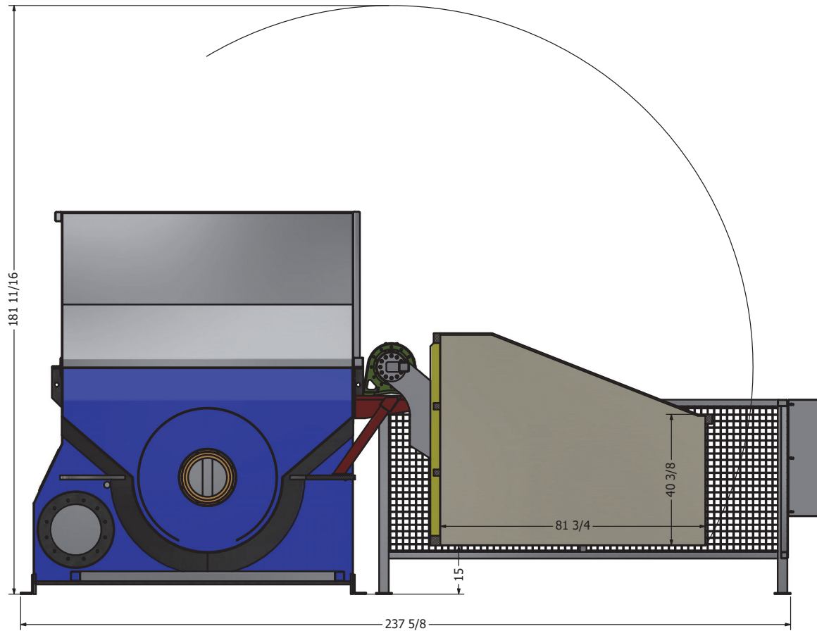
SECTION B-B
